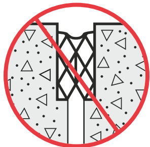
Compression Seal
